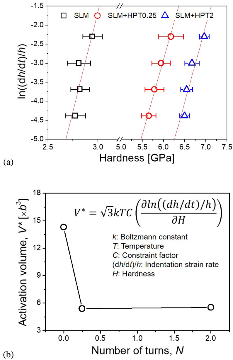
Figure S1 Results of nanoindentation experiments under various indentation strain rate (dh/dt)/h : (a) Logarithmic strain rate versus linear stress; (b) change in activation volume, V^* , upon HPT processing.
